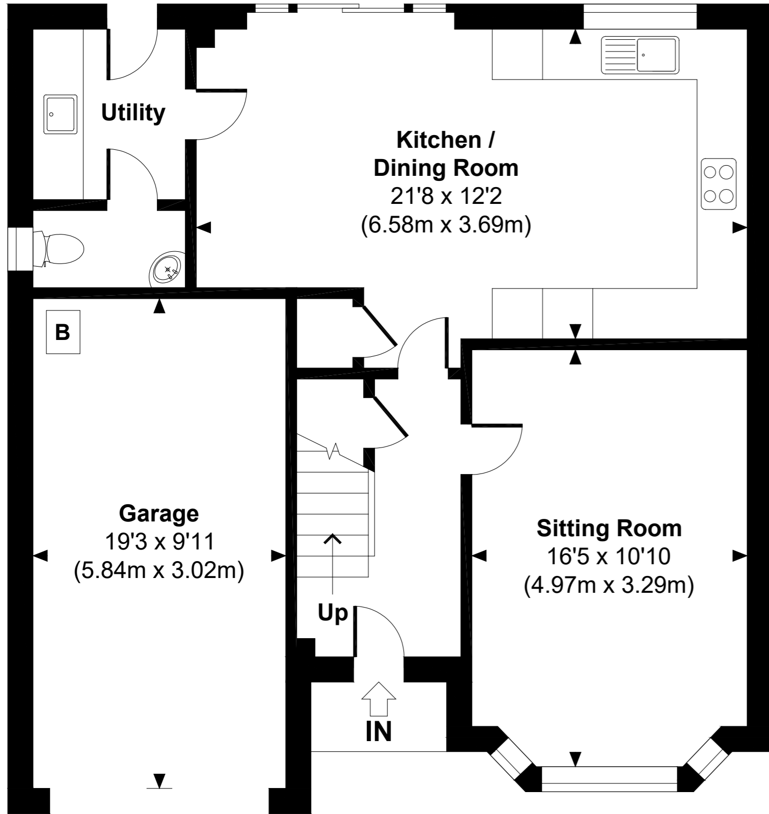
GROUND FLOOR
